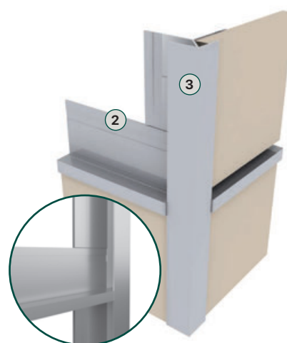
OUTSIDE CORNER
