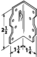
FIGURE 16—AA34
