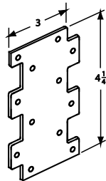
FIGURE 18—ALPT4
