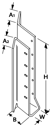
FIGURE 14—ASUR/L HANGERS
