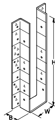
FIGURE 11—AU HANGER ALL OTHER SIZES
