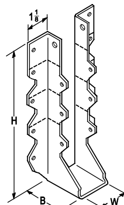
FIGURE 12—AU HANGER 2x SIZES
