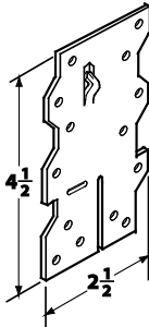
FIGURE 17—AA35F
