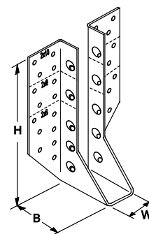
FIGURE 7— AHUS HANGER
