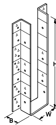
FIGURE 13—AU HANGER ALL OTHER SIZES
