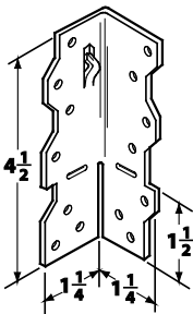
FIGURE 15—AA35
