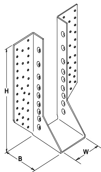
FIGURE 9—AHGUS HANGERS
