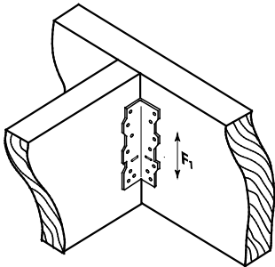
FIGURE 19—TYPICAL INSTALLATION FOR AA34 AND AA35
