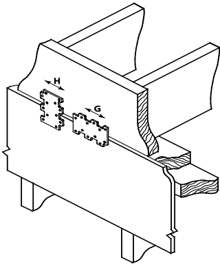
FIGURE 20—TYPICAL INSTALLATION FOR ALPT4 AND AA35F
